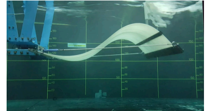
Elastic EEL Energy Tidal Generator
